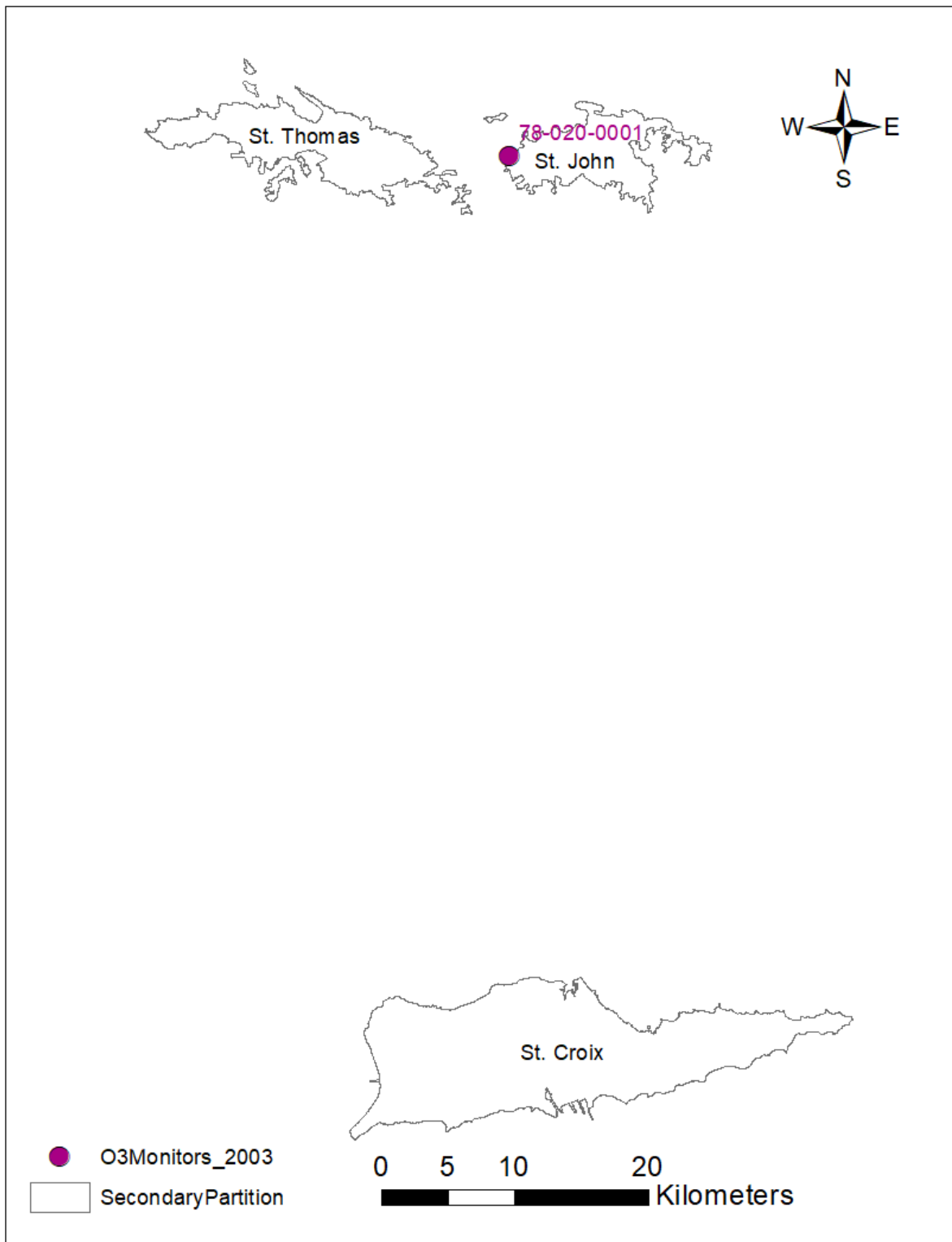
Figure 7 O 3 monitors
