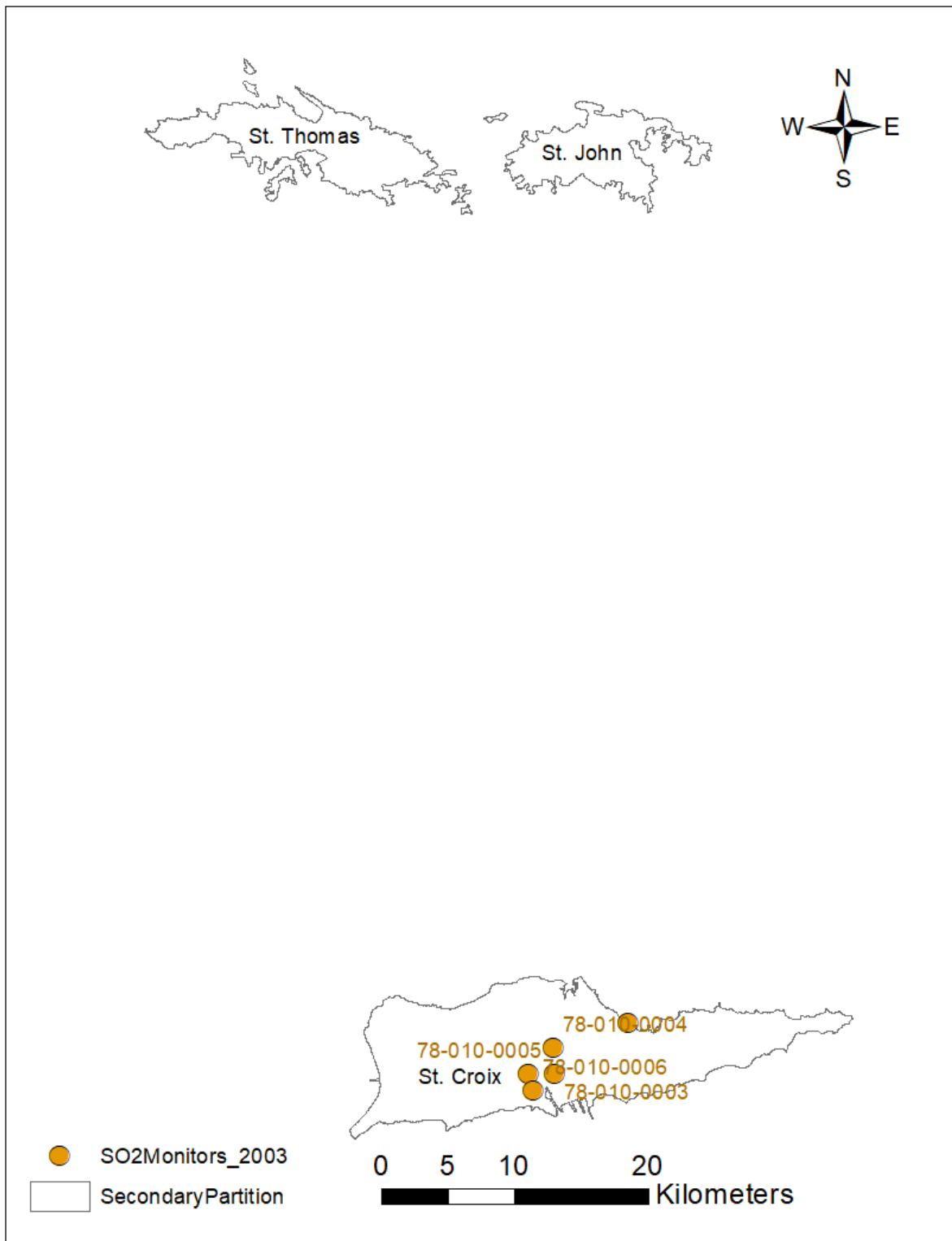
Figure 10 SO 2 monitors
