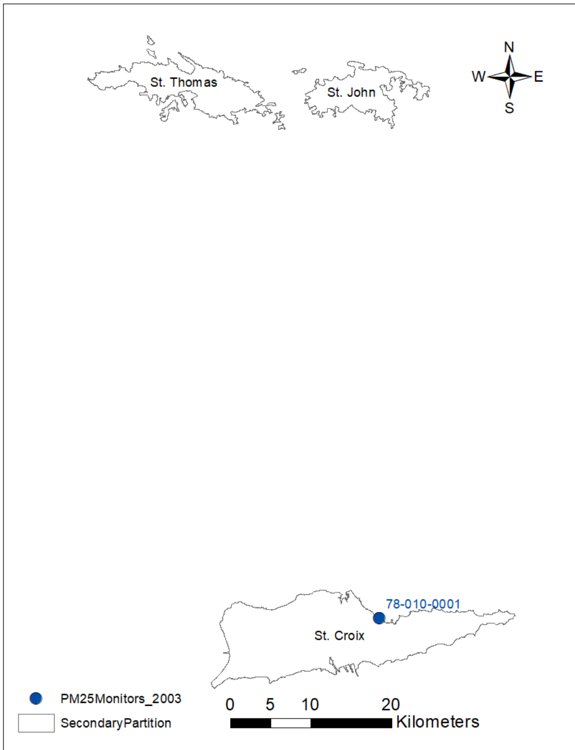
Figure 9 PM 2.5 monitors
