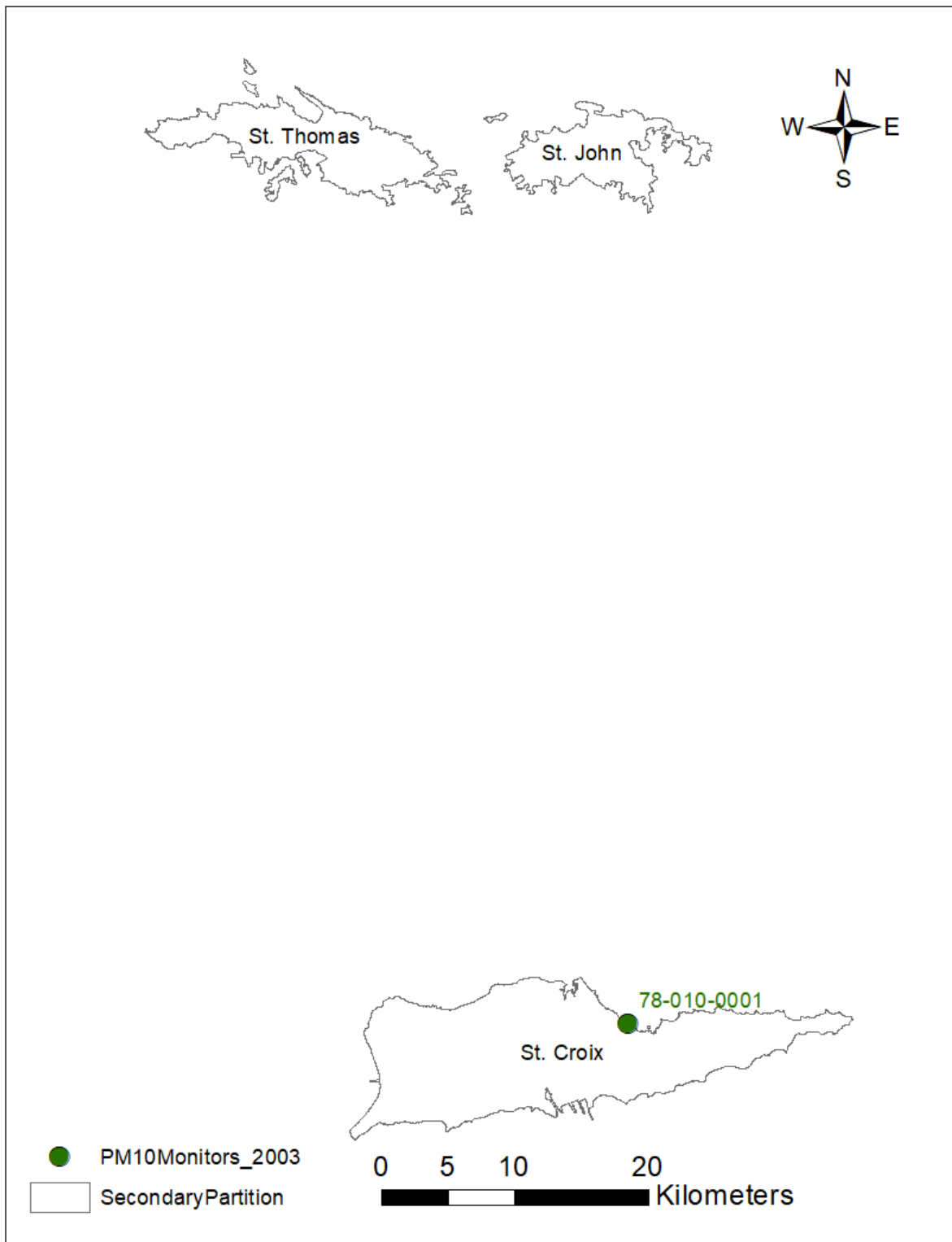
Figure 8 PM 10 monitors
