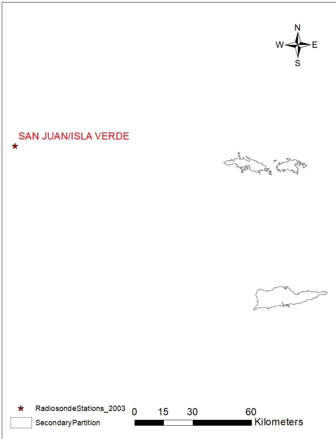
Figure 6 Radiosonde stations
